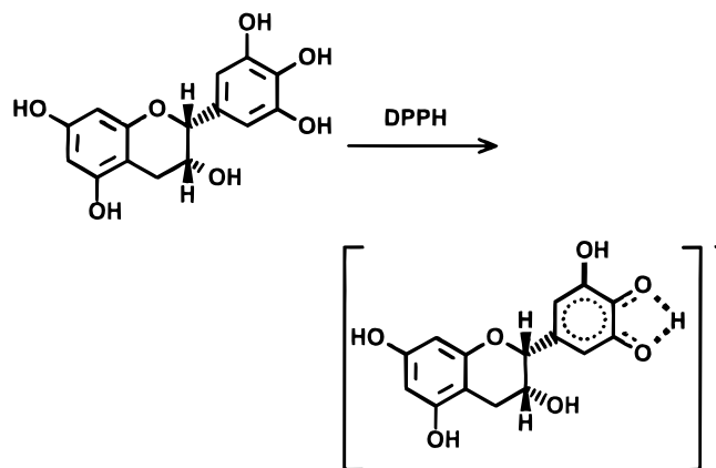
Figure 5. Plausible structure of an (–)-EGC radical generated by DPPH.
