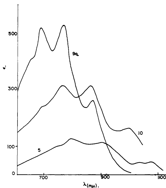
Fig. 2.—The visible and near-infrared spectra of 1,2,5,7-tetramethylcyclohepta[ d,e ]-1-pyridine ( 9a ), 1,2,8-trimethyl-6-isopropylcyclohepta[ d,e ]-1-pyridine ( 10 ), and 2,4-dimethyl-[cyclopentadieno-1',5',4':1,11,10-heptalene] ( 5 ) in saturated hydrocarbon solvent.
