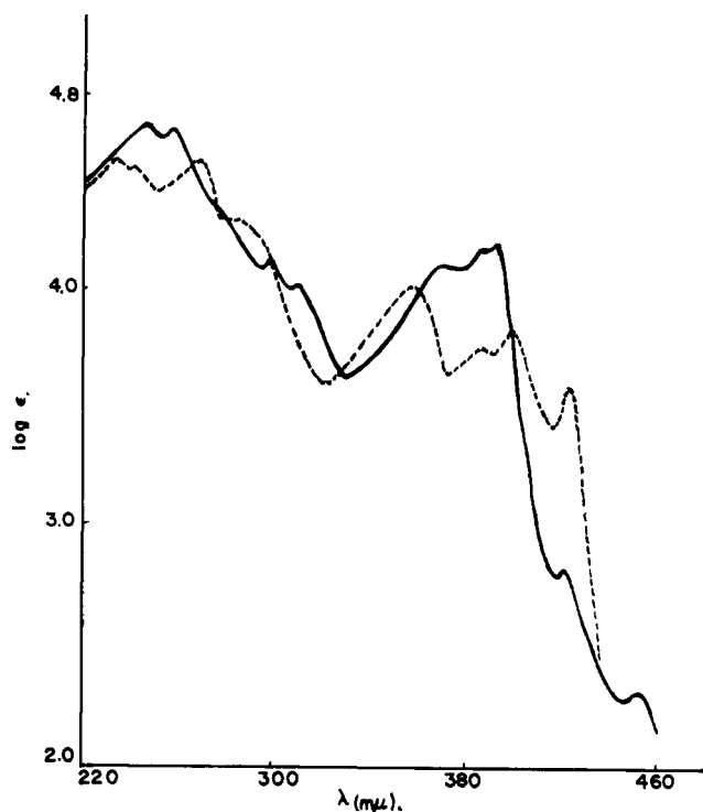
Fig. 1.—The ultraviolet absorption spectra of 1,2,5,7-tetramethylcyclohepta[ d,e ]-1-pyridine (-----) and 2,4-dimethyl-[cyclopentadieno-1',5',4':1,11,10-heptalene] (—) in saturated hydrocarbon solvent.
