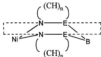
Figure 6. The N 2 E 2 plane in bis(2-pyridyl)borato complexes (E = C, n = 4) and bis(1-pyrazolyl)borato complexes (E = N, n = 3).
