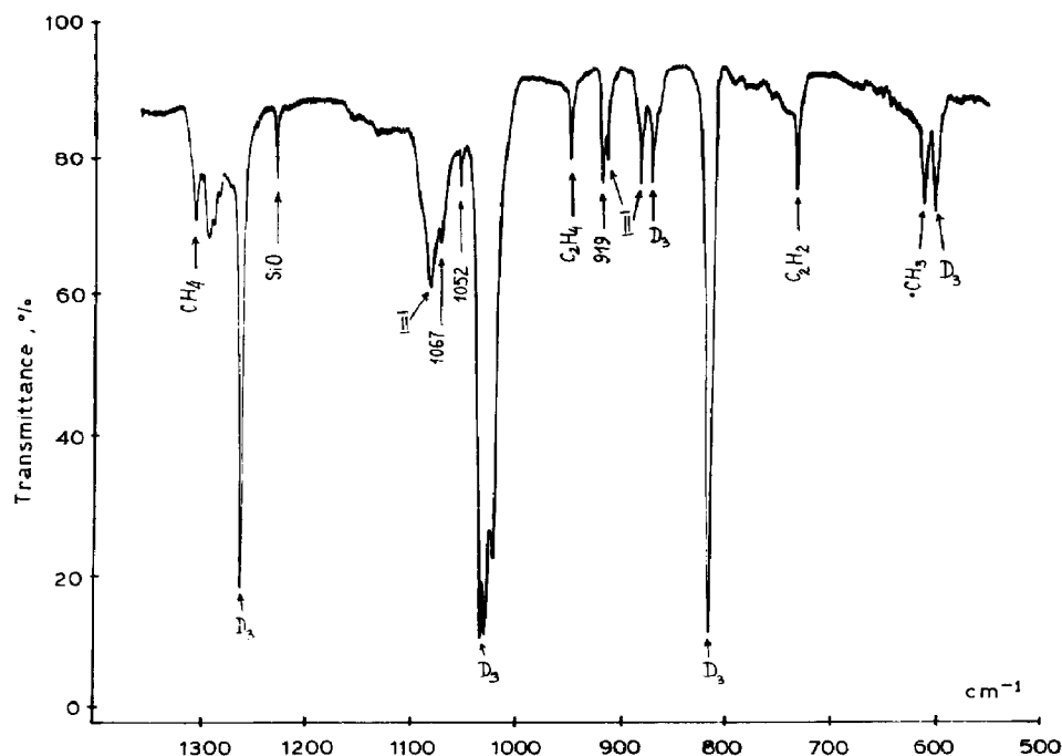
Fig. 1. The matrix IR spectrum (Ar, 12 K) of the vacuum pyrolysis products of octamethylcyclotetrasiloxane (II) at 1030°C and 5 \times 10^{-3} Torr. The bands of the cyclodimer of I, 1,1,3,3-tetramethyl-1,3-cyclodisiloxane (IX), are marked.
