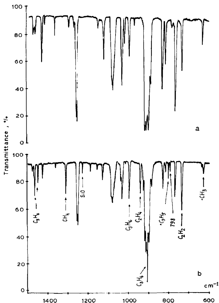
Fig. 2. (a) The matrix IR spectrum (Ar, 12\text{ K} ) of allyloxydimethylsilane (III). (b) IR spectrum of pyrolysis products of III ( 900^\circ\text{C} , 5 \times 10^{-3}\text{ Torr} ), frozen in an Ar matrix at 12\text{ K} .
