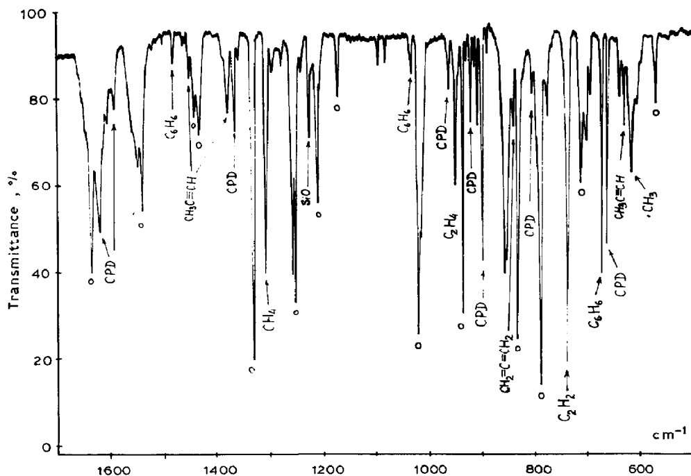
Fig. 4. The matrix IR spectrum (Ar, 12 K) of pyrolysis products of 2,2,6-trimethyl-2-silapyrane (V) at temperature 1050°C and pressure 1 \times 10^{-2} Torr. The bands of the starting compound V (○) and cyclopentadiene (CPD) are marked.
