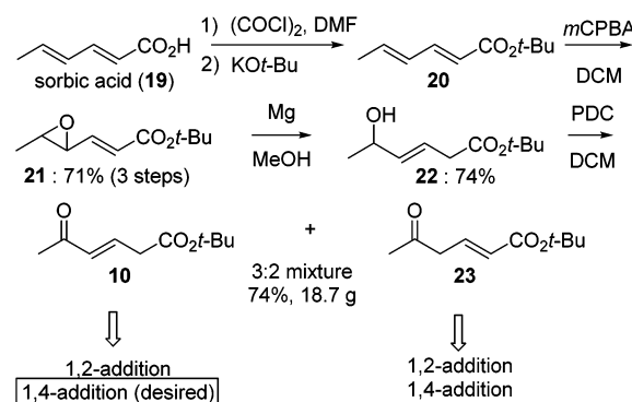
Scheme 4. Synthesis of the Michael Addition Reaction Acceptor 10
