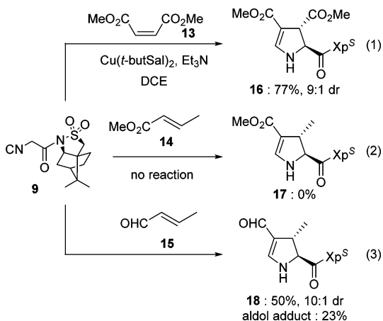
Scheme 3. Michael Addition Cyclization Reaction with 9
