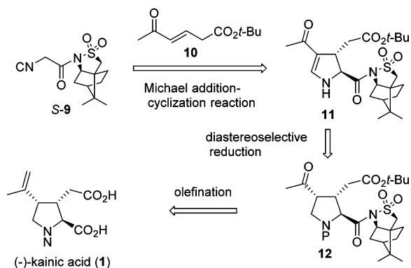
Scheme 2. Synthetic Strategy for the Short Synthesis of Kainic Acid (1)
