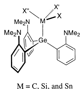
Fig. 1. Ge–M (M = C, Si, and Sn) compounds with three 2-(dimethylamino)phenyl groups.
