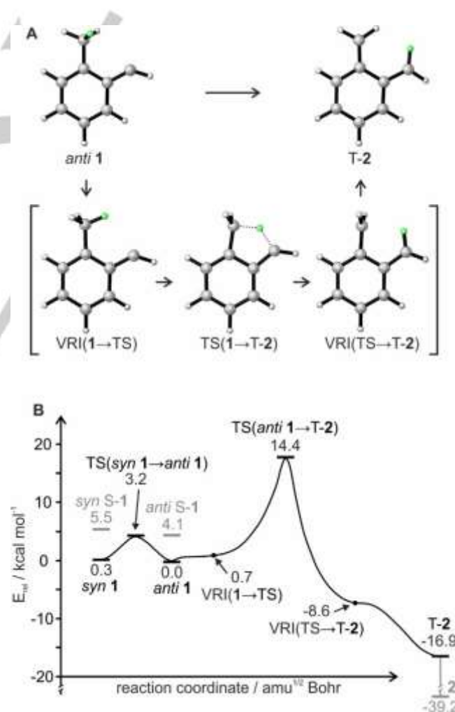
Figure 4. A) Calculated geometries for the tunneling rearrangement of 1. B) Potential energy surface of the syn/anti isomerization of 1 and subsequent rearrangement to 2. The values given are under consideration of the respective zero-point vibrational energies. All calculations were performed at the BLYP-D3/6-311G** level of theory.
