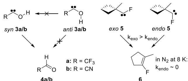
Scheme 2. Examples for conformer-specific hydrogen or carbon tunneling in carbenes: singlet hydroxycarbenes 3a/b [6] and singlet fluorocarbene 5 , respectively. [6]
