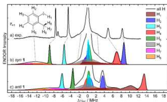
Figure 2. Q-band Davies-type 1 H-ENDOR. a) Experimental spectrum of 1 in MTHF at the z +1 field position of the major spectral contribution of the corresponding EPR spectrum (Figure 1). b, c) Simulations for syn 1 and anti 1 , respectively, employing the g , d and a matrices calculated at the TPSSH-D3/def2-TZVP level of theory (Table S1). Spectra at the x -1 and y -1 positions are shown in Figure S2.
