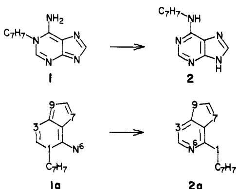
Figure 1. "The clock". Possible routes of the 3-benzyladenine to N^6 -benzyladenine autoclaving rearrangement involving ring opening-reclosure sequences.
