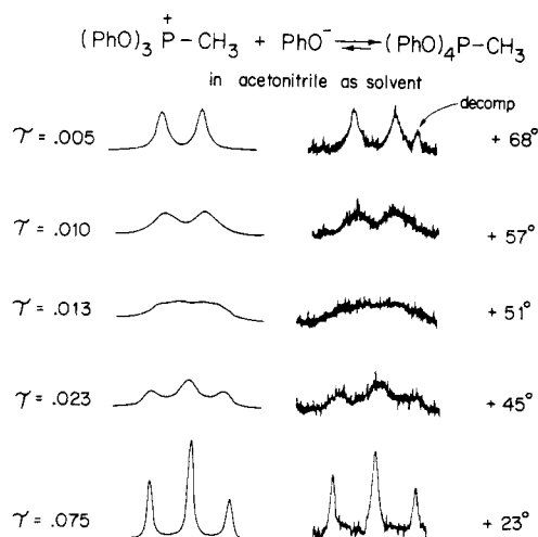
Figure 3. Calculated and observed 60-MHz NMR spectra of a solution of 0.314 M methyltetraphenoxyposphorane and 0.314 M methyltriphenoxyposphonium triflate in acetonitrile- d 3 .
