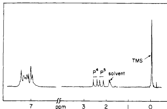
Figure 2. The 100-MHz ^1\text{H} NMR spectrum of an equimolar mixture of methyltetraphenoxyposphorane and methyltriphenoxyphosphonium triflate in acetonitrile- d_3 .
