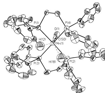
Figure 1. ORTEP drawing (50% probability ellipsoids) of [\text{MnCO}(\text{dppe})_2]^+ . Selected bond lengths (Å): \text{Mn}(1)-\text{C}(50) , 1.733(7); \text{Mn}(1)-\text{P}(1) , 2.278(2); \text{Mn}(1)-\text{P}(2) , 2.280(2); \text{Mn}(1)-\text{P}(3) , 2.321(2); \text{Mn}(1)-\text{P}(4) , 2.335(2); \text{Mn}(1)-\text{H}(12) , 2.89(6); \text{Mn}(1)-\text{H}(18) , 2.98(6). Selected bond angles (deg): \text{C}(50)-\text{Mn}(1)-\text{P}(1) , 92.3(2); \text{C}(50)-\text{Mn}(1)-\text{P}(2) , 90.8(2); \text{C}(50)-\text{Mn}(1)-\text{P}(3) , 96.1(2); \text{C}(50)-\text{Mn}(1)-\text{P}(4) , 97.2(2); \text{P}(1)-\text{Mn}(1)-\text{P}(4) , 82.67(7); \text{P}(2)-\text{Mn}(1)-\text{P}(3) , 82.90(7); \text{P}(1)-\text{Mn}(1)-\text{P}(3) , 95.68(7); \text{P}(2)-\text{Mn}(1)-\text{P}(4) , 98.02(7).
