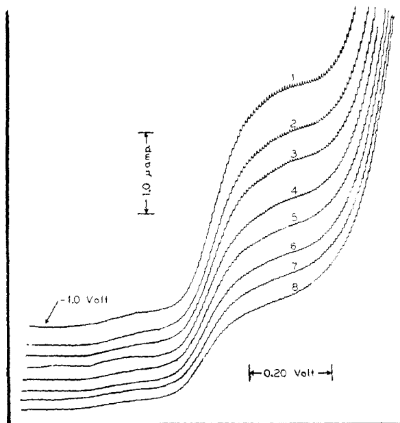
Fig. 1.—Polarograms of streptomycin A in phosphate buffer pH 10.6 at 65°; the i_d for polarogram 1 was recorded 10.0 minutes after the addition of the streptomycin A to the phosphate buffer solution; the time interval between polarograms was 5.0 minutes.
