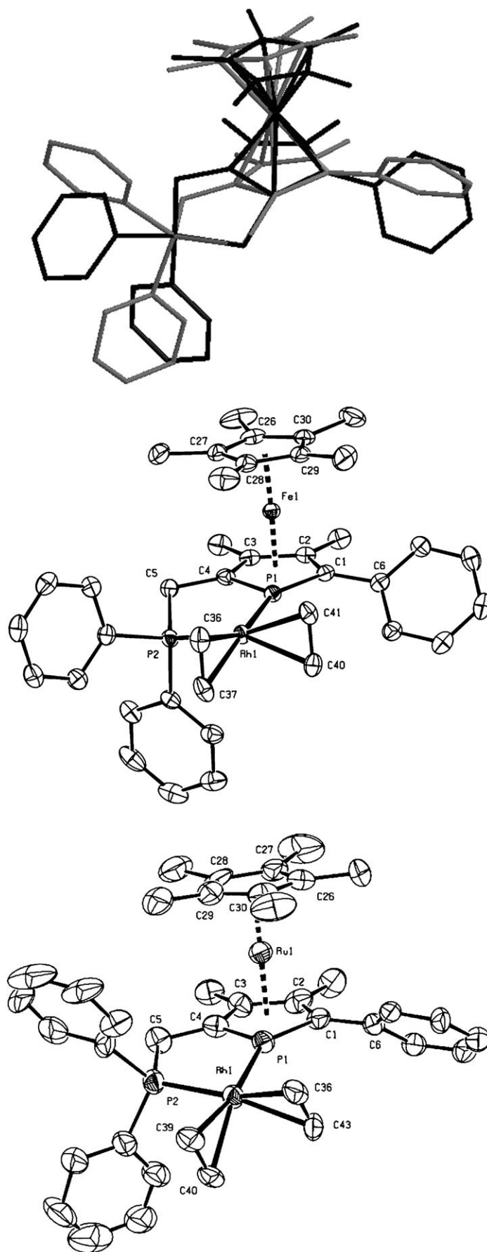
Figure 3. Configurational assignment of 16 . Bond lengths (expressed as an average of the two molecules in the unit cell): Ru1–P1 2.398(1), Ru1–C1 2.228(5), Ru1–C2 2.195(4), Ru1–C3 2.186(5), Ru1–C4 2.205(6), P1–C1 1.787(5), P1–C4 1.777(6), P2–C10 1.820(5), C1–C2 1.442(8), C2–C3 1.429(7), C3–C4 1.439(8), P2–C5 1.843(5), P2–B1 1.927(9) Å.
