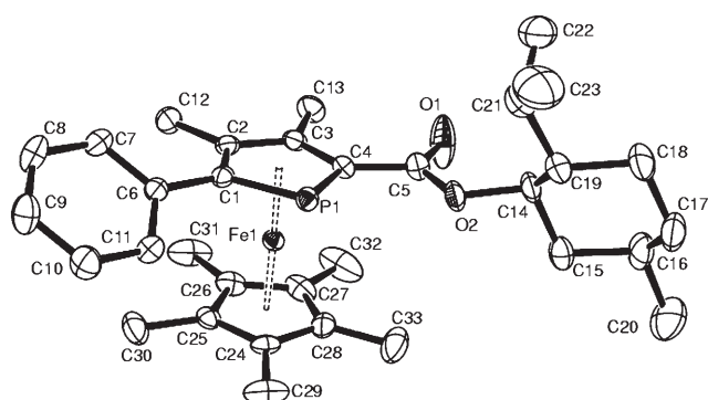
Figure 1. Left: Structure of the ( R_{\text{Fc}} ) diastereomeric phosphaferrrocene precursor 9 (orange-red hexagons) employed in this study. Selected bond lengths: Fe1–C3 2.067(2), Fe1–C2 2.083(2), Fe1–C1 2.102(2), Fe1–P1 2.289(1), P1–C4 1.785(2), P1–C1 1.785(2), C1–C2 1.434(2), C2–C3 1.423(2), C2–C12 1.510(2), C3–C4 1.433(2), C3–C13 1.501(2), C4–C5 1.479(2) Å. Right: Structure of diastereomeric phosphaferrrocene ( S_{\text{Fc}} )- 9a (orange-red rhomboids). Selected bonds lengths from one of two very similar molecules in the unit cell: Fe1–C3 2.056(3), Fe1–C4 2.068(3), Fe1–C2 2.080(3), Fe1–C1 2.094(4), Fe1–P1 2.291(1), P1–C4 1.783(3), P1–C1 1.784(3), C1–C2 1.418(5), C2–C3 1.435(5), C3–C4 1.434(5), C4–C5 1.473(5) Å.
