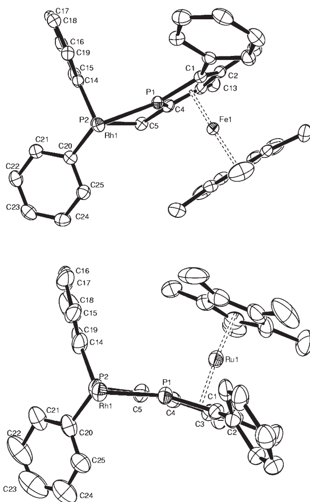
Figure 5. Complexes ( \pm )- 18 (top) and (+)- 19 (bottom) as viewed down the \text{Rh-P}(\text{sp}^3) bond, showing how retention of a given chirality at the \text{PPh}_2 function upon passing from \text{M}=\text{Fe} to \text{M}=\text{Ru} requires inversion at the phosphametalocene component. The \text{BF}_4^- counterion and cod are omitted. Note that the (–)-phosphoferrocene enantiomer is shown, rather than the (+)-hand employed in the catalysis.
