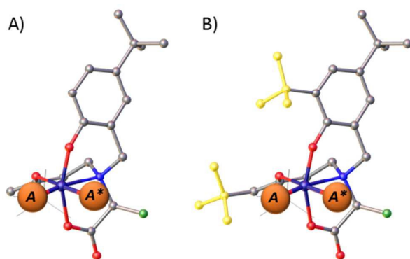
Figure 3. Models showing the achiral ( A ) and chiral ( A* ) sites for: A) S - 13 B) S - 14 ; constructed using a mononuclear unit from the asymmetric unit of 12 3 (HOiPr). A portion of the model is displayed as wireframe for clarity. Yellow: tert -butyl groups in the R'' positions. Green: methyl group in the X position. Orange: achiral ( A ) and chiral ( A* ) sites. Purple: titanium. Grey: carbon. Blue: nitrogen. Red: oxygen.
