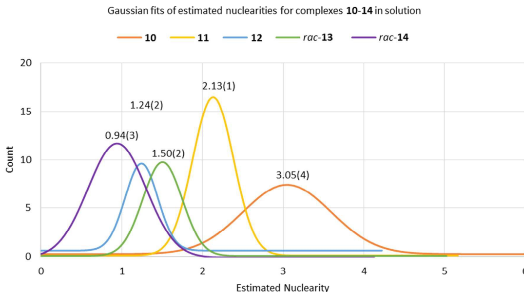
Figure 2. Plot of Gaussian fitting curves for datasets of estimated nuclearities of 10-14 in CDCl 3 versus the count of data points corresponding to said nuclearity. The estimated nuclearities were obtained by 1 H DOSY NMR experiments via estimated MWs. See Supporting Information for further details.
