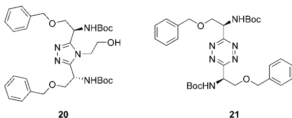
FIGURE 1. Triazole ( 20 ) and tetrazine ( 21 ) impurities resulting from amidrazones dimerization.
