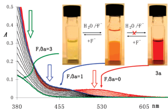
Figure 2. The MLCT region of the UV-vis titration spectra of 3a ( 3.2 \times 10^{-5} M) by TBAF in \text{CH}_2\text{Cl}_2 . The red region corresponds to the spectral change with the addition of 1 equiv of \text{F}^- . Inset: visual color change of 3a ( 1.0 \times 10^{-3} M) with the addition of 1 equiv of \text{F}^- (middle) and 3 equiv of \text{F}^- in \text{CH}_2\text{Cl}_2 and the reverse color switching after addition of \text{H}_2\text{O} (middle).
