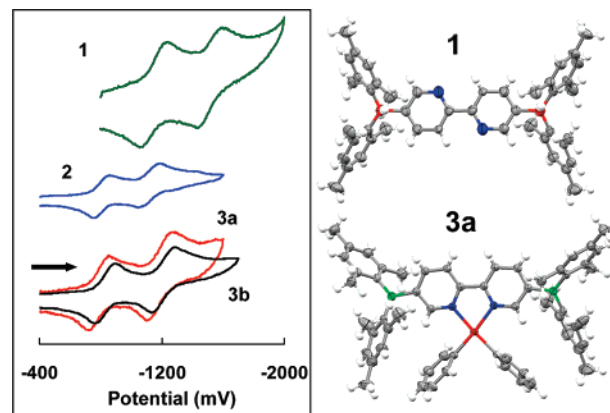
Figure 1. Left: cyclic voltammograms of 1 , 2 , 3a , and 3b versus Ag/AgCl reference electrode ( E_{1/2}^{\text{ox}} of FeCp 2 = 0.55 V) in DMF (0.10 M NBu 4 PF 6 , scan rate = 2 V/s for 1 and 3a and 0.5 V/s for 2 and 3b ). Right: crystal structures of 1 and 3a .
