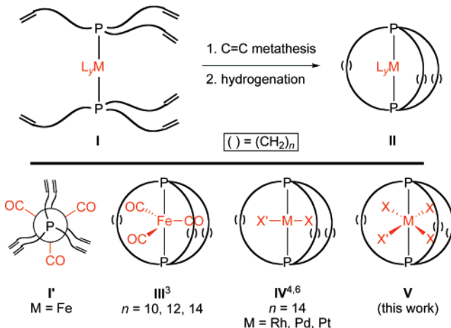
Scheme 1. Previous Syntheses of Gyroscope-Like Complexes in Which trans -Phosphorus Atoms Are Linked by Three Aliphatic Bridges
