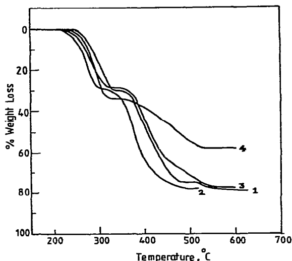
Fig. 3. Thermal decomposition curves of oxalato(heeen) complexes. 1, \text{Mn(heeen)}_2\text{C}_2\text{O}_4 ; 2, \text{Cu(heeen)}_2\text{C}_2\text{O}_4 ; 3, \text{Zn(heeen)}_2\text{C}_2\text{O}_4 ; 4, \text{Cd(heeen)C}_2\text{O}_4 .
