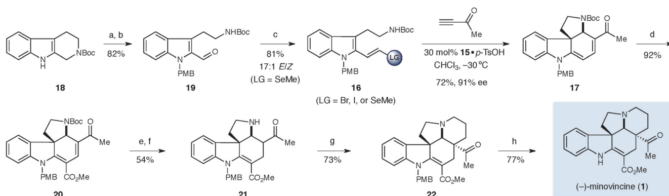
Scheme 2. Total synthesis of (–)-minovincine: a) NaH, PMBCl, DMF, 0 °C, 94 %; b) SeO 2 , 95:5 1,4-dioxane/H 2 O, 100 °C, 87 %; c) LG = Br: [(PPh 3 )CH 2 Br] 2 Br, tBuOK, THF, –78 °C, 21 %; LG = I: CrCl 2 , CHI 3 , THF, 0 °C, 50 %; LG = SeMe: (EtO) 2 P(O)CH 2 SeMe, KHMDs, [18]crown-6, –78 °C to RT, 81 %; d) N -iodosuccinimide, [Pd(PhCN) 2 Cl 2 ] (10 mol %), Et 3 N, MeOH, MeCN, CO (1 atm), 60 °C, 92 %; e) L -Selectride, THF, –78 to 0 °C, 75 %; f) (Me) 3 SiH, Et 3 N, CH 2 Cl 2 , 0 °C, 72 %; g) 1,3-diiodopropane, NaHCO 3 , DMF, 35 °C; then tBuOK, tBuOH, RT, 73 %; h) 1:1 TFA/CH 2 Cl 2 , 0 °C to RT, 77 %. DMF = N,N -dimethylformamide, HMDs = hexamethyldisilazide, TFA = trifluoroacetic acid, THF = tetrahydrofuran, Ts = 4-toluenesulfonyl.
