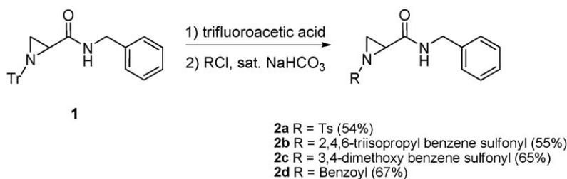
Scheme 1. Preparation of aziridine-based model compounds 2a–d .
