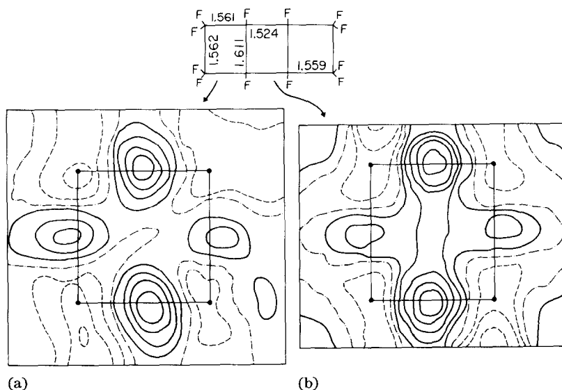
Fig. 2. Deformation electron density sections for cyclobutane fragments of tricyclo-octane (5): (a) peripheral cycle; (b) central cycle. Interval between isolines, 0.1 \text{ e } \text{\AA}^{-3} .
