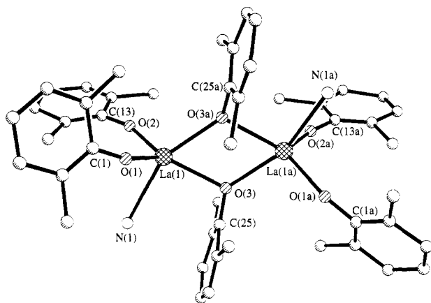
Figure 2. Ball-and-stick representation emphasizing the oxygen-bridged dimeric structure of \text{La}_2(\text{O}-2,6\text{-}i\text{-Pr}_2\text{C}_6\text{H}_3)_6(\text{NH}_3)_2 ( 3 ). Methyl carbon atoms of the isopropyl groups have been omitted for clarity.
