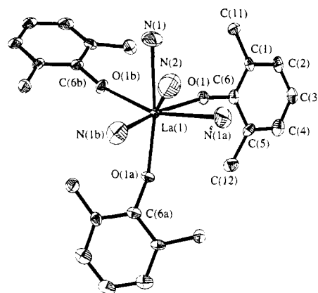
Figure 3. ORTEP representation (50% probability ellipsoids) of the capped octahedral coordination geometry of \text{La}(\text{O}-2,6\text{-}i\text{-Pr}_2\text{C}_6\text{H}_3)_3(\text{NH}_3)_4 ( 4 ), giving the atom numbering scheme used in the tables. Methyl carbon atoms of the isopropyl groups have been omitted for clarity.
