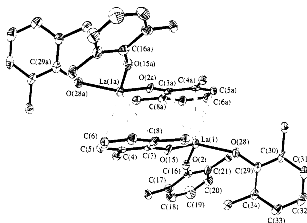
Figure 1. ORTEP plot (50% probability ellipsoids) showing the centrosymmetric η-arene-bridged dimeric structure of La 2 (O-2,6- i -Pr 2 C 6 H 3 ) 6 ( 2 ) and giving the atom numbering scheme used in tables. Methyl carbon atoms of the isopropyl groups have been omitted for clarity.
