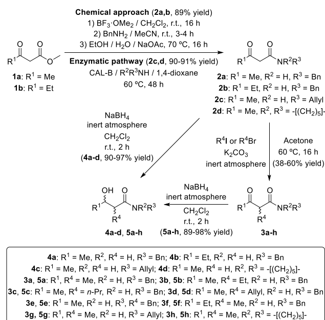
Scheme 1. Synthesis of ( \alpha -substituted) \beta -keto amides and racemic \beta -hydroxy amides.
