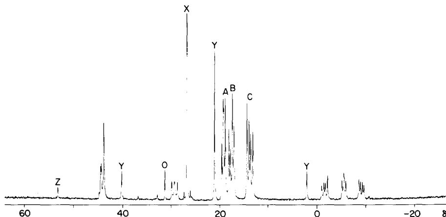
Fig. 2. ^{31}\text{P}\{^1\text{H}\} NMR spectrum (80.98 MHz) of \text{Pt}(\text{PPh}_3)_2(\text{SP}) at -117^\circ\text{C} in \text{THF-}d_8 . Peaks marked X, Y and Z are probably due to \text{Ph}_3\text{PO} , \text{Pt}(\text{SP})_2 and \text{Pt}(\text{PPh}_3)_3 respectively; O arises from an unknown impurity.
