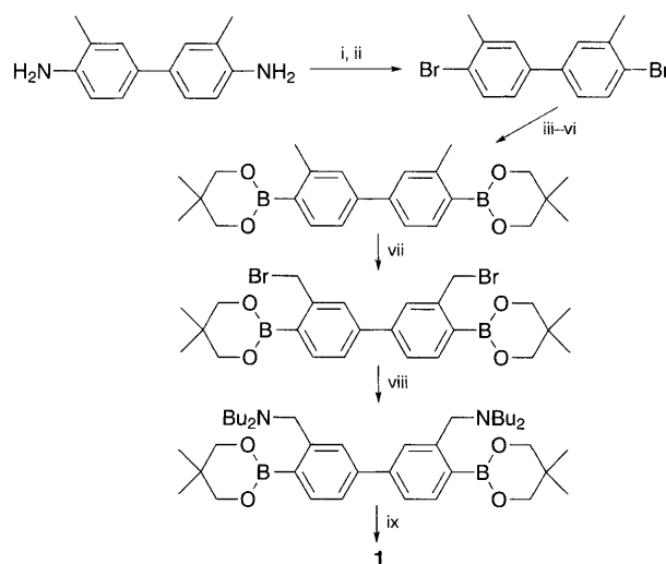
Scheme 1 Reagents and conditions (yields): i, NaNO 2 , 50% H 2 SO 4 ; ii, CuBr, 47% HBr (30%); iii, butyllithium, THF, -78 °C; iv, B(OMe) 3 , THF, -78 °C; v, 2 mol dm -3 HCl, room temp.; vi, 2,2-dimethyl-1,3-propanediol, toluene, reflux (35%); vii, NBS, CCl 4 (76%); viii, Bu 2 NH, K 2 CO 3 , MeCN, room temp. (93%); ix, dil. HCl, CHCl 3 , room temp. (41%)
