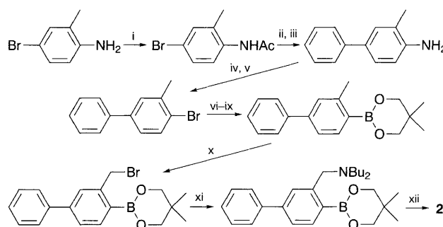
Scheme 2 Reagents and conditions (yields): i, AcCl, Et 3 N, CH 2 Cl 2 , 0 °C (95%); ii, Pd(PPh 3 ) 4 , PhB(OH) 2 , Na 2 CO 3 , 80 °C (87%); iii, 2 mol dm -3 HCl, reflux (97%); iv, NaNO 2 , 50% H 2 SO 4 ; v, CuBr, 47% HBr (35%); vi, butyllithium, THF, -78 °C; vii, B(OMe) 3 , THF, -78 °C; viii, 2 mol dm -3 HCl, room temp.; ix, 2,2-dimethylpropane-1,3-diol, toluene, reflux (82%); x, NBS, CCl 4 (87%); xi, Bu 2 NH, K 2 CO 3 , MeCN, room temp. (72%); xii, Na 2 CO 3 aq., Et 2 O, room temp.
