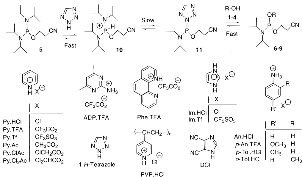
Figure 1. General structure of activators studied.
