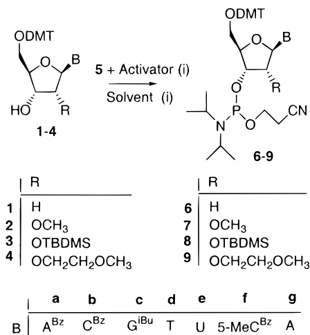
Scheme 1. Synthesis of phosphoramidites
