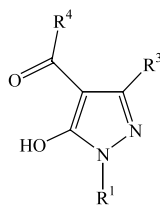
Fig. 1. 4-Acyl-pyrazol-5-one prolignands LH.
