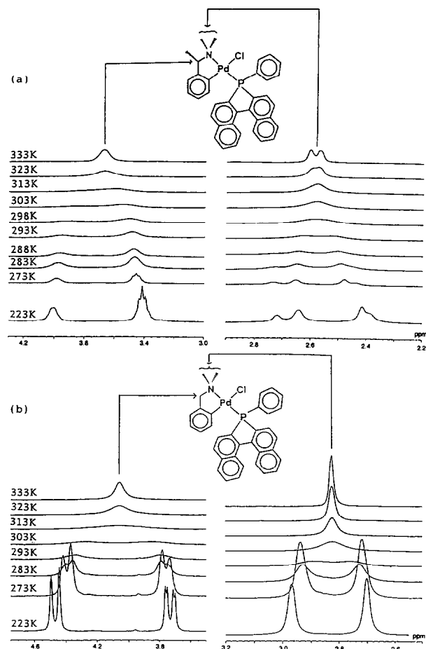
Fig. 4. Temperature-dependent 1 H NMR spectra (270.05 MHz): (a) for NMe 2 and CH protons of (S)(P)-4a; (b) for NMe 2 and CH 2 protons of 4b. In CDCl 3 .
