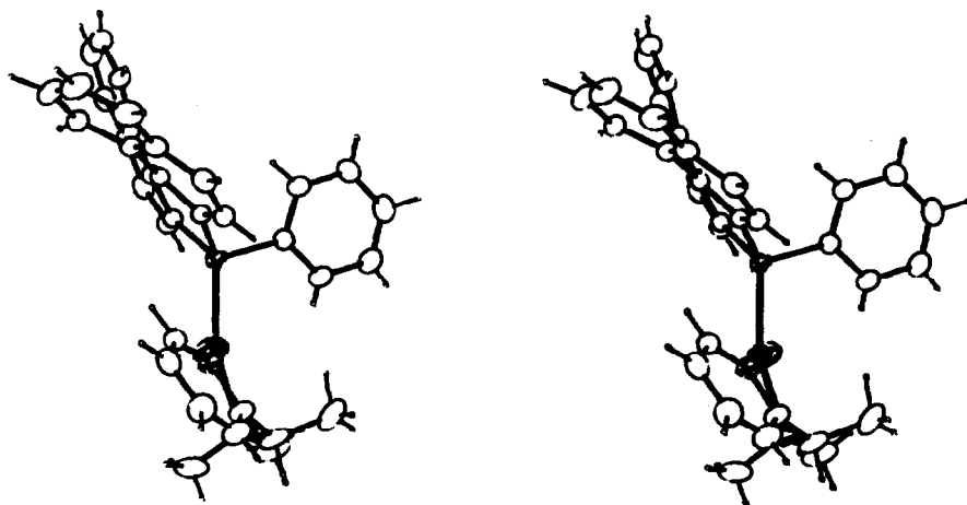
Fig. 2. Stereososcopic drawing of the molecule of (S)(P) -4a.
