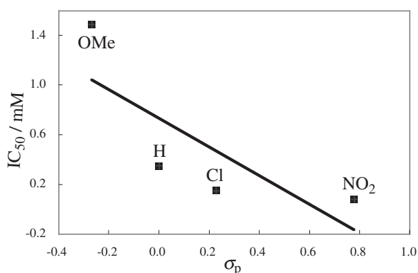
Figure 1. The relationship between IC 50 values and the Hammett's substituent constants.
