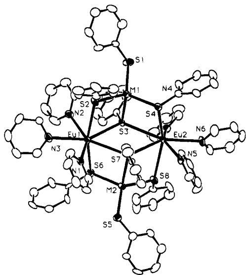
Figure 1. Molecular structures of [(py)_3Eu(\mu_2-SPh)_2(\mu_3-SPh)M(SPh)]_2 \cdot 2 py (compound 1 , M = Hg ; compound 2 , M = Cd ). The tetrametallic clusters contain 7-coordinate Eu ions and 4-coordinate group II metal ions, connected by \mu_2 and \mu_3 benzenethiolate ligands. The lattice pyridine has been omitted for clarity. Thermal ellipsoids (ORTEP) are drawn at the 50% probability level ( M = Cd ).
