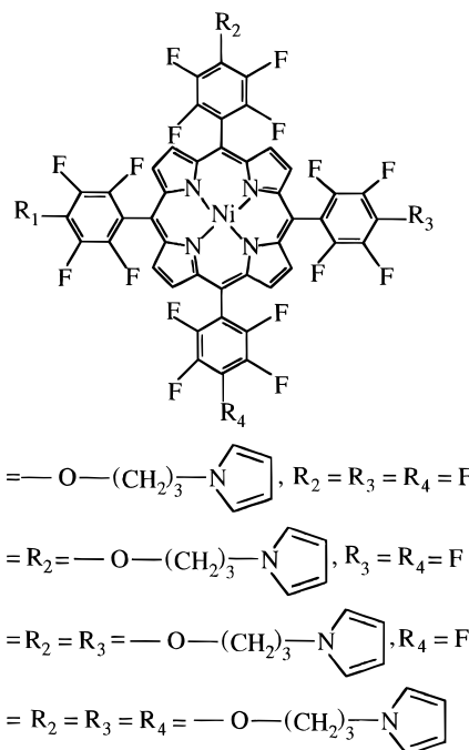
Figure 1. Structures of the 1a–d compounds.
