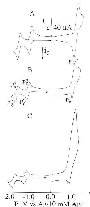
Figure 3. Cyclic voltammograms recorded at a glassy carbon electrode (diameter 5 mm) of (A) NiTFPP, (B) 1a monomer, and (C) 1d monomer in \text{CH}_3\text{CN} + 0.1 M TBAP. Scan rate = 0.1 \text{ V s}^{-1} .
