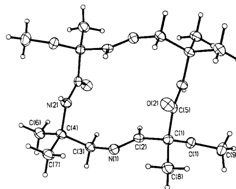
Figure 1. Compound 6aa .
