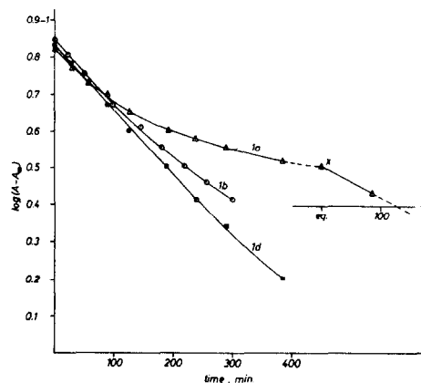
Figure 1. First order rate plots \log(A-A_\infty) vs. time for reaction (2) at 80^\circ\text{C} with \text{L} = \text{P}(\text{C}_6\text{H}_5)_3 (see text and Table III).
