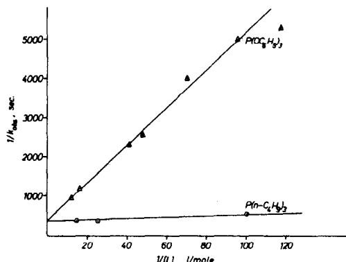
Figure 2. Plot of the reciprocal of the observed rate constants vs. the reciprocal of the concentration of L for reaction (15).
