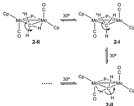
Scheme 4. Dynamic Process Proposed for Compound 2 in Solution (Substituents on Phosphorus Omitted for Clarity; Only the First Steps Shown)
