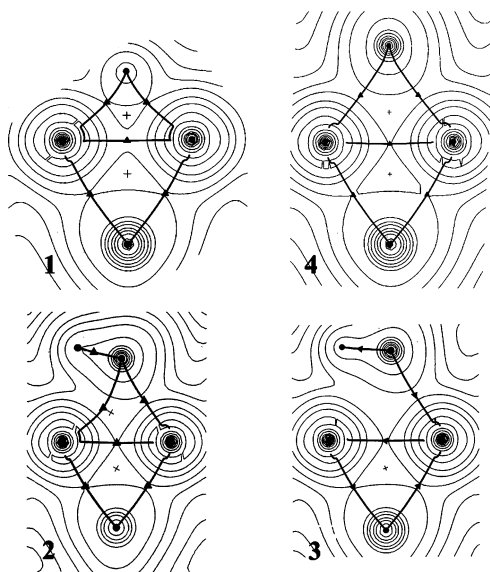
Figure 8. Contour lines of the electron density (B3LYP) in the plane \text{Mo}_2\text{P} of compounds 1–4, showing the bond paths linking the bond critical points ( \blacktriangle ) and the corresponding atoms ( \bullet ), as well as the ring critical points ( \times ).
