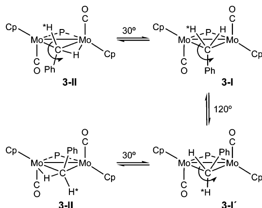
Scheme 3. Fluxionality and Isomerization Processes Proposed for Compound 3 in Solution (Substituents on Phosphorus Omitted for Clarity)
