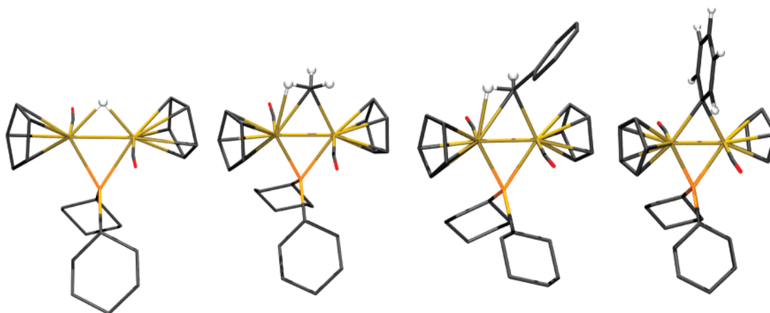
Figure 5. Optimized structures (B3LYP) for compounds 1–4.
