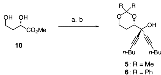
Scheme 3. (a) 2-Methoxypropene, PPTS, acetone, 84% or \text{Ph}_2\text{C}(\text{OMe})_2 , p -TsOH, benzene, 74%; (b) n\text{-BuC}\equiv\text{CH} , \text{EtMgBr} , THF, 92% for 5 and 79% for 6 . PPTS = pyridinium p -toluenesulfonate.
