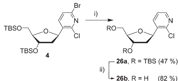
Scheme 7 Reagents and conditions: (i) vinyl \text{MgBr} , \text{Fe}(\text{acac})_3 , rt, 12 h; (ii) \text{Et}_3\text{N}\cdot 3\text{HF} , THF, rt, 14 h.
