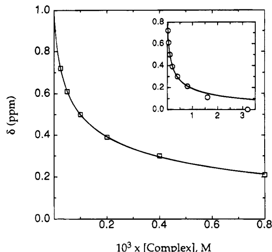
Figure 3. Concentration dependence of ^1\text{H} NMR chemical shift for the methyl group of [\text{Pt}(\text{terpy})\text{Me}]\text{Cl} in \text{D}_2\text{O} at 298 K (see text for details).
