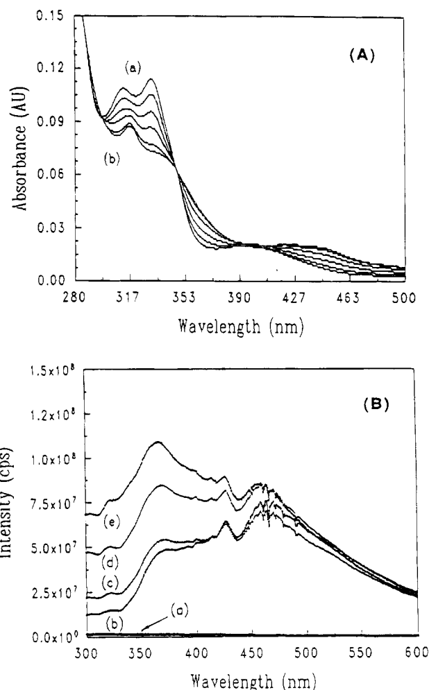
Figure 4. (A) Spectral changes associated with the addition of calf thymus DNA to a solution of [\text{Pt}(\text{terpy})\text{Me}]\text{Cl} in buffer D at 25 °C. Experimental conditions: (a) [\text{complex}] = 12.5 \mu\text{M} ; (b) [\text{DNA}] = 0.6, 1.8, 3.0, 3.6, 4.7 \mu\text{M} . (B) Resonance light-scattering profiles: (a) 1 mM phosphate buffer; (b) 12.5 \mu\text{M} [\text{Pt}(\text{terpy})\text{Me}]\text{Cl} ; after the addition of ct -DNA, (c)–(e) [\text{DNA}] = 0.6, 3.0, 4.7 \mu\text{M} .
