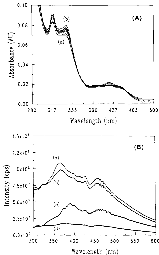
Figure 5. (A) Spectral changes associated with the addition of calf thymus DNA to a solution of [Pt(terpy)Me]Cl in buffer D at 25 °C. Experimental conditions: (a) [complex] = 12.5 \mu M; (b) [DNA] = 27.6, 36.2, 44.4, 63.7, 81.4, 112.7, 139.5 \mu M. (B) Resonance light-scattering profiles of 12.5 \mu M [Pt(terpy)Me]Cl after the addition of ct -DNA: (a)–(d) [DNA] = 4.7, 8.5, 44.4, 81.4 \mu M.
