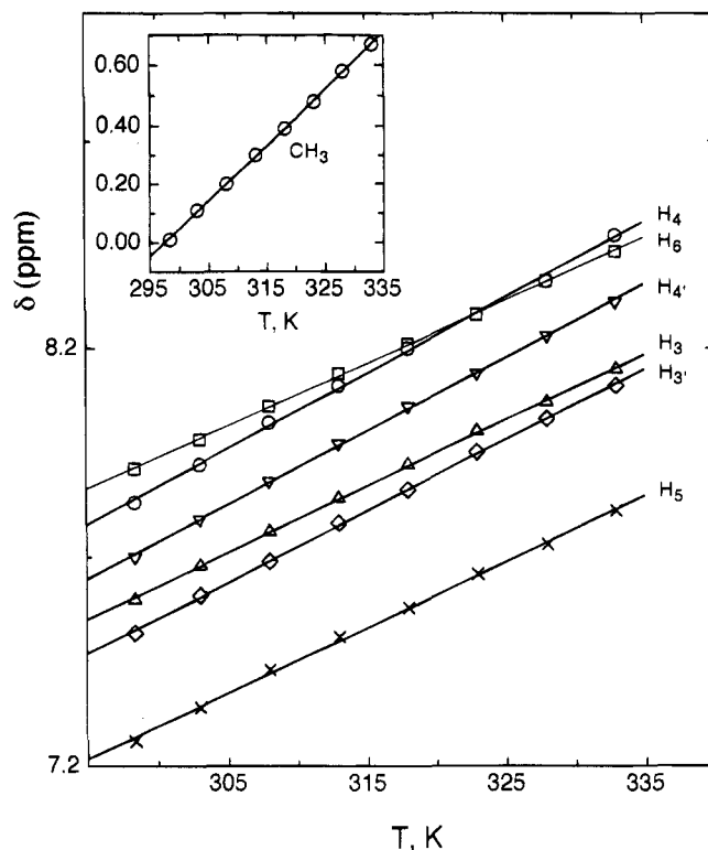
Figure 2. 300.13 MHz ^1\text{H} NMR chemical shift temperature dependence of [\text{Pt}(\text{terpy})\text{Me}]\text{Cl} in \text{D}_2\text{O} ([complex] = 0.01 M).
