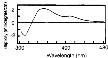
Figure 6. CD spectra of [Pt(terpy)Me]Cl in the presence of ct -DNA. Experimental conditions: [complex] = 0.05 mM; [DNA] = 1 mM in buffer A at 298 K.
