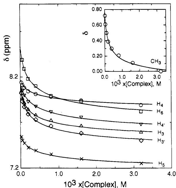
Figure 1. Concentration dependence of ^1\text{H} NMR resonances of [\text{Pt}(\text{terpy})\text{Me}]\text{Cl} in \text{D}_2\text{O} at 298 K.
