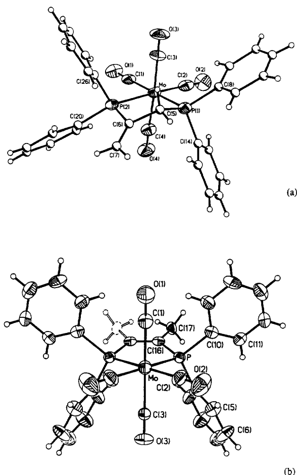
Fig. 2. Structural drawings of (a) 5 and (b) 6 showing the atom numbering scheme (40% probability ellipsoids). Hydrogen atoms have an arbitrary radius of 0.1 Å.
