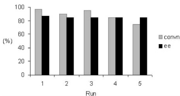
Figure 3. Proof of recoverability of 5 (up to five times) in the catalytic enantioselective condensation of MeNO 2 with PhCHO.
