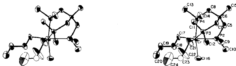
Fig. 1. Stereo ORTEP drawing of the nonhydrogen atoms of Cr( n -Bu) 2 Cl[(Me 2 PCH 2 ) 3 CMe], showing atom labeling. Only one occupied site for the disordered carbon (C23) is shown.
