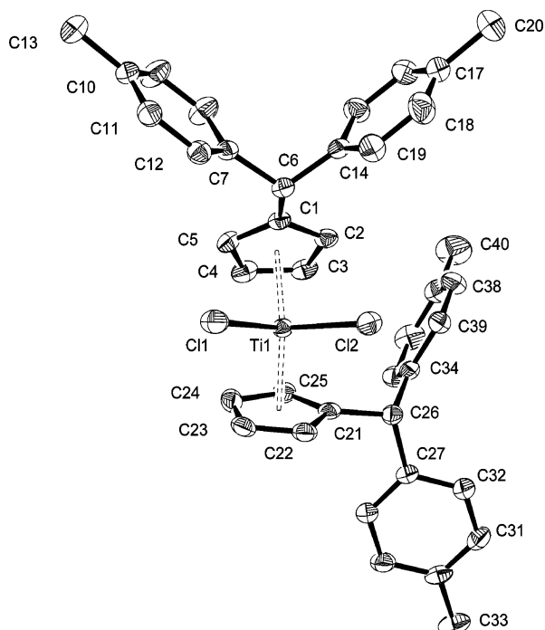
Figure 11. Molecular structure of 9 (50% probability ellipsoids). Selected bond lengths (Å) and angles (deg): Ti1–C1 = 2.4475(15), Ti1–C2 = 2.4149(15), Ti1–C3 = 2.3532(16), Ti1–C4 = 2.3416(15), Ti1–C5 = 2.3977(15), Ti1–C21 = 2.4117(16), Ti1–C22 = 2.4279(16), Ti1–C23 = 2.4152(16), Ti1–C24 = 2.3386(17), Ti1–C25 = 2.3632(17), Ti1–Cl1 = 2.3506(5), Ti1–Cl2 = 2.3397(5), C1–C6 = 1.507(2), C21–C26 = 1.510(2), Ti1–Ct1 = 2.070, Ti1–Ct2 = 2.070; Ct1–Ti1–Ct2 = 132.6, Cl1–Ti1–Cl2 = 95.32. Ct1 = centroid of C1–C5; Ct2 = centroid of C21–C25.
