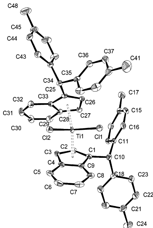
Figure 12. Molecular structure of 10 (50% probability ellipsoids). Selected bond lengths (Å) and angles (deg): Ti1–C1 = 2.493(2), Ti1–C2 = 2.355(2), Ti1–C3 = 2.308(2), Ti1–C4 = 2.552(2), Ti1–C9 = 2.626(2), Ti1–C25 = 2.450(2), Ti1–C26 = 2.373(2), Ti1–C28 = 2.494(2), Ti1–C33 = 2.521(2), C1–C10 = 1.512(3), C25–C34 = 1.508(3), Ti1–Cl1 = 2.3026(6), Ti1–Cl2 = 2.3192(6), Cl1–Ti–Cl2 = 97.61(3), Ct1–Ti–Ct2 = 131.69(2). Ct1 = centroid of C1–C4, C9; Ct2 = centroid of C25–C28, C33.
