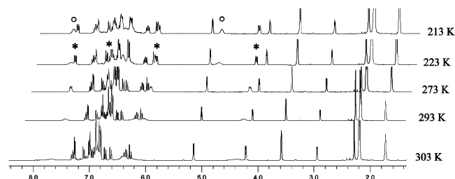
Figure 10. Variable-temperature ^1\text{H} NMR spectra of 7 in \text{THF-}d_8 (300.1 MHz). The asterisks mark the resonances of the protons from ring D, and the circles denote the C–H resonances of ring C (two of them are overlapped by the aromatic region).
