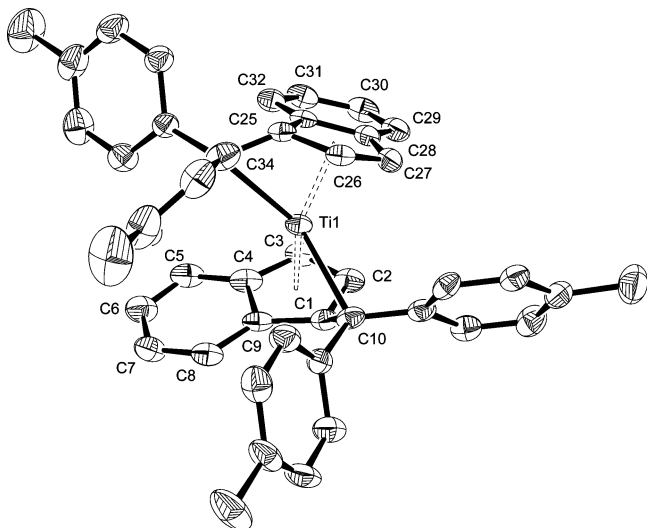
Figure 3. Molecular structure of ( S,pS,pR )- 7 (50% probability ellipsoids). Selected bond lengths (Å) and angles (deg): Ti1–C1 = 2.155(3), Ti1–C2 = 2.225(3), Ti1–C3 = 2.342(3), Ti1–C4 = 2.488(3), Ti1–C9 = 2.365(3), Ti1–C10 = 2.400(2), C1–C2 = 1.445(4), C2–C3 = 1.407(5), C3–C4 = 1.420(5), C4–C9 = 1.440(4), C4–C5 = 1.414(5), C5–C6 = 1.354(5), C6–C7 = 1.424(4), C7–C8 = 1.362(4), C1–C9 = 1.457(4), C1–C10 = 1.456(4), Ti1–C25 = 2.146(3), Ti1–C26 = 2.235(3), Ti1–C27 = 2.409(3), Ti1–C28 = 2.497(3), Ti1–C33 = 2.328(3), Ti1–C34 = 2.410(3), C25–C26 = 1.449(4), C26–C27 = 1.379(5), C27–C28 = 1.420(4), C28–C33 = 1.420(4), C28–C29 = 1.419(4), C29–C30 = 1.359(4), C30–C31 = 1.397(5), C31–C32 = 1.369(4), C32–C33 = 1.429(4), C25–C34 = 1.425(4), Ti1–Ct1 = 1.972, Ti1–Ct2 = 1.983; Ct1–Ti1–Ct2 = 142.9, C10–Ti1–C34 = 126.64(9). Ct1 = centroid of C1–C4, C9; Ct2 = centroid of C25–C28, C33.
