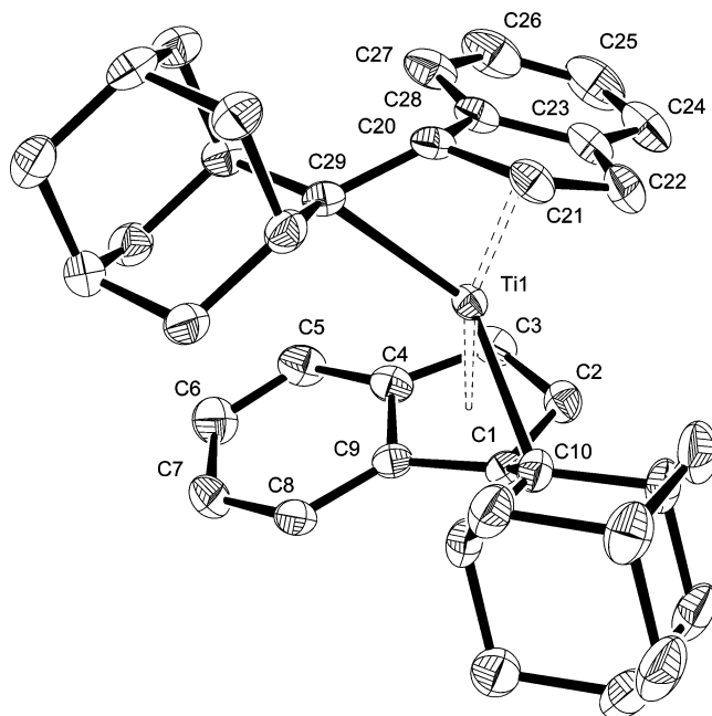
Figure 4. Molecular structure of 8 (50% probability ellipsoids, ( S,pS,pR ) enantiomer shown). Selected bond lengths (Å) and angles (deg): Ti1–C1 = 2.146(2), Ti1–C2 = 2.233(2), Ti1–C3 = 2.257(2), Ti1–C4 = 2.529(2), Ti1–C9 = 2.415(2), Ti1–C10 = 2.341(2), C1–C2 = 1.449(3), C2–C3 = 1.400(3), C3–C4 = 1.429(3), C4–C9 = 1.436(3), C4–C5 = 1.420(3), C5–C6 = 1.372(3), C6–C7 = 1.412(3), C7–C8 = 1.374(3), C1–C9 = 1.479(3), Ti1–C20 = 2.138(2), Ti1–C21 = 2.259(2), Ti1–C22 = 2.411(2), Ti1–C23 = 2.4964(18), Ti1–C28 = 2.345(2), Ti1–C29 = 2.363(2), C20–C21 = 1.440(3), C21–C22 = 1.403(3), C22–C23 = 1.426(3), C23–C28 = 1.438(3), C23–C24 = 1.429(3), C24–C25 = 1.362(4), C25–C26 = 1.406(4), C26–C27 = 1.379(4), C27–C28 = 1.423(3), Ti1–Ct1 = 1.988, Ti1–Ct2 = 1.995; Ct1–Ti1–Ct2 = 143.2, C10–Ti1–C2 = 9 120.09(8). Ct1 = centroid of C1–C4, C9; Ct2 = centroid of C20–C23, C28.
