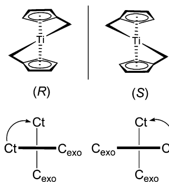
Figure 6. Chirality of the bis(fulvene) complexes. Ct = centroid of the five membered fulvene ring; \text{C}_{\text{exo}} = exocyclic carbon atom of the fulvene ligand.
