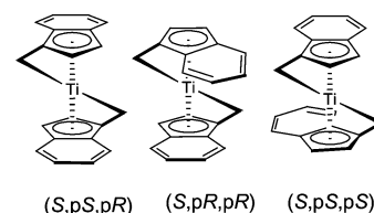
Figure 7. Diastereomers of the bis(benzofulvene) complexes (only one enantiomer given for each). 16
