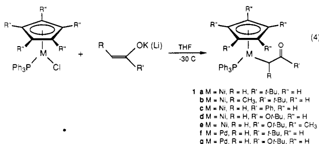
Scheme II
