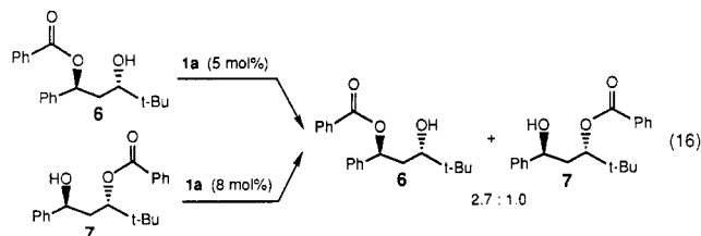
Scheme VII
