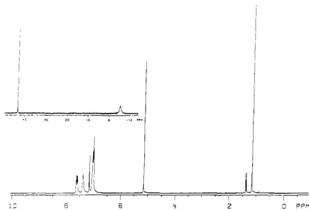
Figure 2. ^1\text{H} and ^{31}\text{P}\{^1\text{H}\} (inset) NMR spectra of \text{Cp}(\text{Ph}_3\text{P})\text{NiCH}_2\text{CO}-t\text{-Bu} and \text{Ph}_3\text{P} in \text{C}_6\text{D}_6 .
