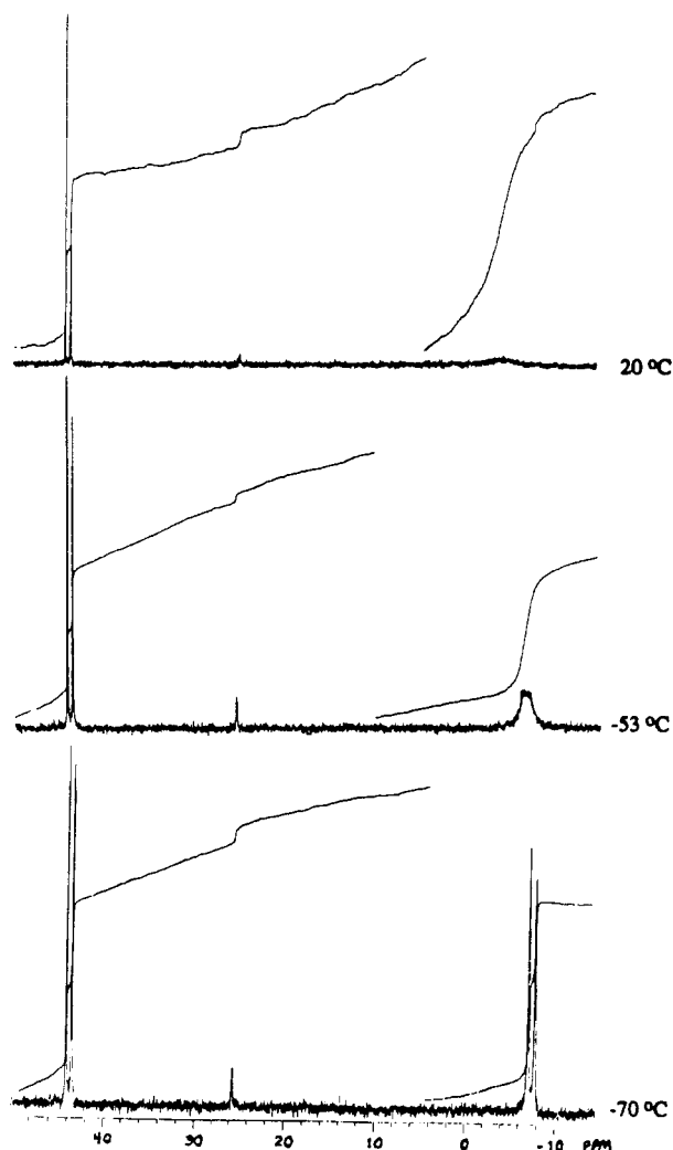
Figure 3. Variable-temperature ^{31}\text{P}\{^1\text{H}\} NMR spectrum of \text{Cp}(\text{Ph}_3\text{P})_2\text{NiCH}_2\text{CO}-t\text{-Bu} ( d_0 and d_{15} ) and \text{Ph}_3\text{P} ( d_0 and d_{15} ).
