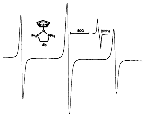
Figure 5. X-Band EPR spectrum of \text{Cp}(\text{Ph}_2\text{PCH}_2\text{CH}_2\text{PPh}_2)\text{Ni}(1) in THF at 22^\circ\text{C} ( g = 2.050 , a = 0.0120\text{ cm}^{-1} ) with the following parameters of modulation amplitude (G), microwave power (dB), and receiver gain: 10, 12, 4.0 \times 10^4 . The DPPH resonance (external standard, g = 2.0037 ) is included on the spectrum.
