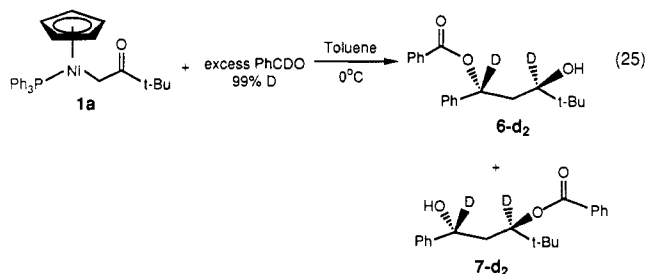
Scheme X
