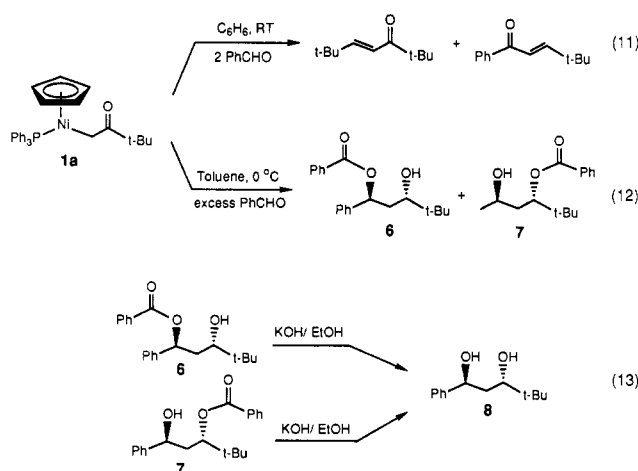
Scheme V
