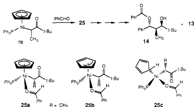
Scheme XII
