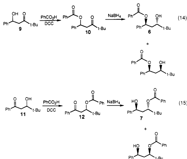
Scheme VII
