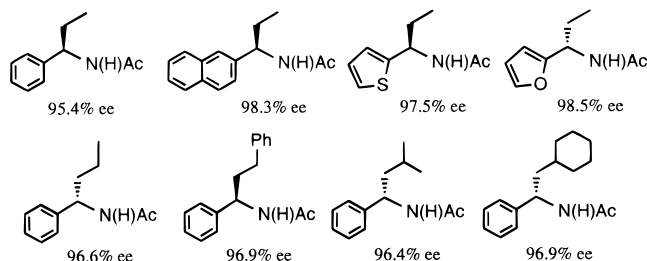
Figure 1. Asymmetric catalytic synthesis of \alpha -arylalkylamine derivatives. (R)- (S)-amines derived from (R,R)-Me-BPE-Rh and (S,S)-Me-DuPHOS-Rh catalysts, respectively.
