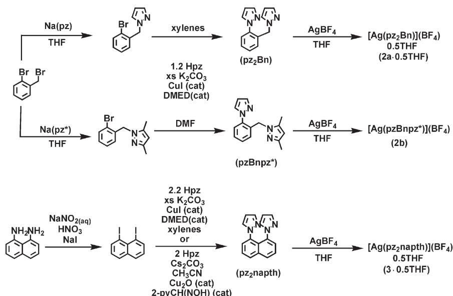
Scheme 1. Syntheses of Dipyrzolyloxyorganyls and Their Silver(I) Complexes
