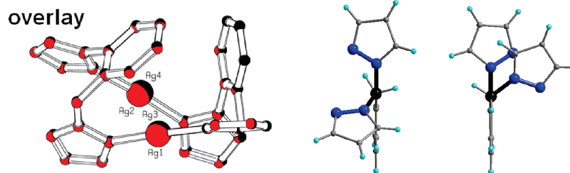
Figure 7. Overlay of two crystallographically independent cyclic dications in 2a ·0.5acetone (left) with views of gauche,syn (center) and staggered,syn (right) ligand conformations that occur within each cyclic dication.
