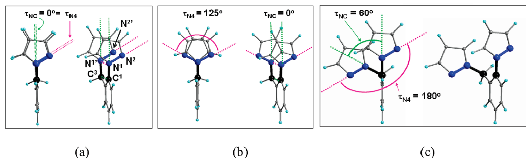
Figure 3. Two spacer-independent torsion angles, \tau_{N4} ( N^2N^1-N^1N^{2'} , pink) and \tau_{NC} ( N^1C^1-C^3N^{1'} , green), for describing the relative conformations of pyrazolyls using pz 2 Bn with coplanar pyrazolyls as an example (two views of the molecule are given for each conformation): (a) eclipsed, \text{syn-}\tau_{N4} = \tau_{NC} = 0^\circ ; (b) eclipsed, \text{anti-}\tau_{N4} = 125^\circ , \tau_{NC} = 0^\circ ; (c) staggered, \text{anti-}\tau_{N4} = 180^\circ , \tau_{NC} = 60^\circ . See the text for comments on the carbon hybridization.
