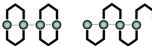
Figure 2. Possible supramolecular isomers of 1:1 metal complexes of bridging multinucleating ligands (ligands are in black and metals in gray). Left: Cyclic structures. Right: Polymeric structures.
