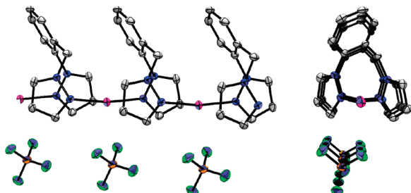
Figure 6. Two views of the coordination polymer chain of 2a . Left: Chain propagating along the b axis. Right: View of the chain down the b axis.
