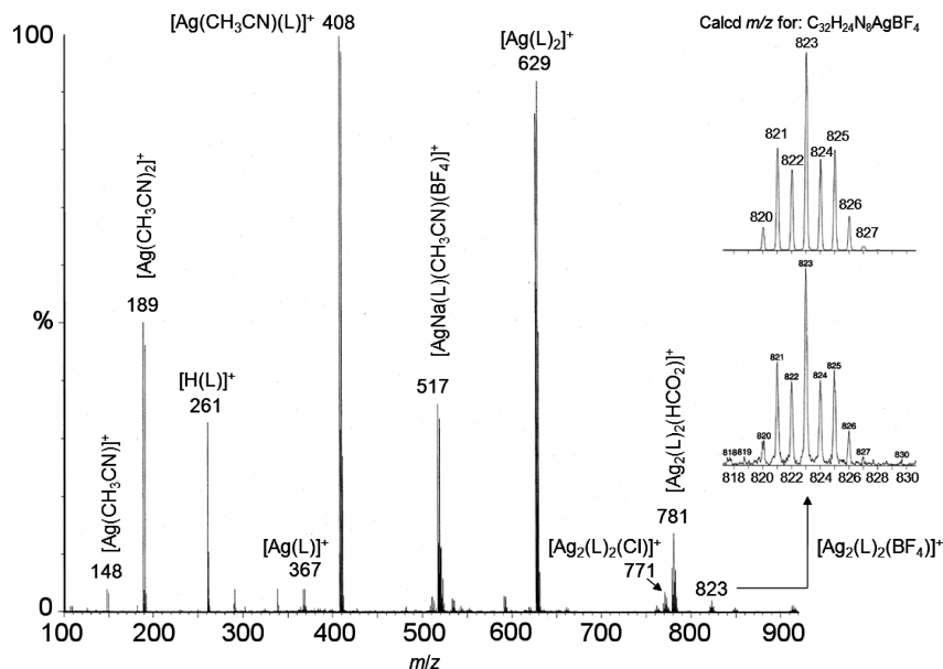
Figure 11. Representative ESI(+)-MS of 3·0.5THF in acetonitrile.
