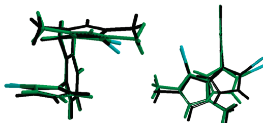
Figure 8. Overlay of cationic monomer units in 2b (black) and 2b ·acetone (green) with silver in cyan.
