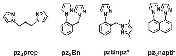
Chart 1. Dipyrazolylorganyl Ligands Investigated in This Study
