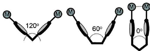
Figure 1. Expected geometries for metals (M) binding to tethered monodentate heterocycles with unspecified Lewis donor atoms (black spheres) containing one-atom (left), two-atom (center), and three-atom spacers (right).
