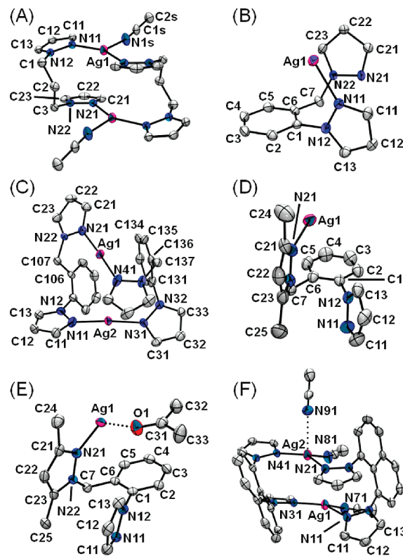
Figure 4. ORTEP diagrams (thermal ellipsoids drawn at the 50% probability level) and atom labeling of cyclic disilver dications or monomeric cation units of silver coordination polymers. (A) 1 ·CH 3 CN; (B) 2a ; (C) 2a ·0.5acetone; (D) 2b ; (E) 2b ·acetone; (F) 3 ·2CH 3 CN.
