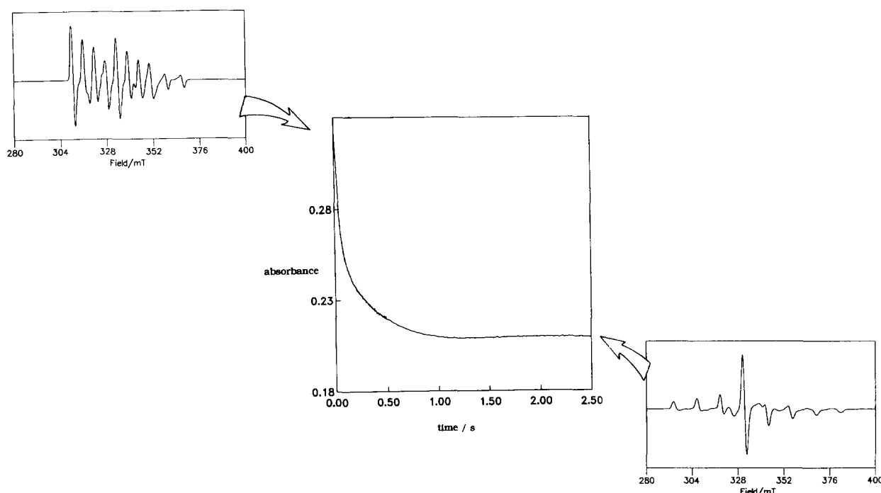
Fig. 1. Centre—Typical stopped-flow absorbance–time curve for the reaction of [\text{V}(\eta^5\text{-C}_5\text{H}_5)_2(\eta^2\text{-PhCCPh})] ( 0.25 \text{ mmol dm}^{-3} ) with anhydrous \text{HCl} ( 10.0 \text{ mmol dm}^{-3} ) in \text{thf} at 25.0^\circ\text{C} , measured at \lambda = 420 \text{ nm} . Left—EPR spectrum of [\text{V}(\eta^5\text{-C}_5\text{H}_5)_2(\eta^2\text{-PhCCPh})] in \text{thf} . Right—EPR spectrum of the product of the reaction between [\text{V}(\eta^5\text{-C}_5\text{H}_5)_2(\eta^2\text{-PhCCPh})] and anhydrous \text{HCl} in \text{thf} . This spectrum is essentially identical to that of an authentic sample of [\text{V}(\eta^5\text{-C}_5\text{H}_5)_2\text{Cl}_2] .
