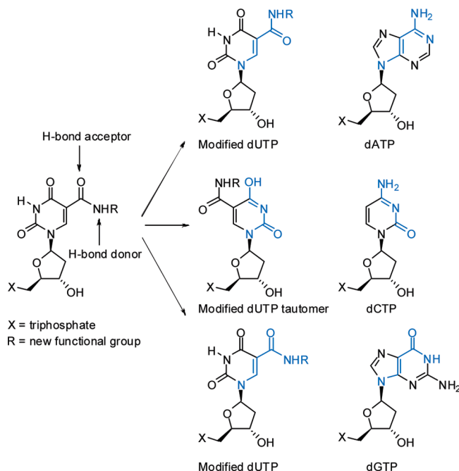
Figure 2. Some possible orientations of 5-position modifications on dUTP that lead to new H-bonding motifs. Atoms and bonds shown in blue indicate highly similar regions where a modified dUTP could present itself almost identically to each of the native nucleotides.
