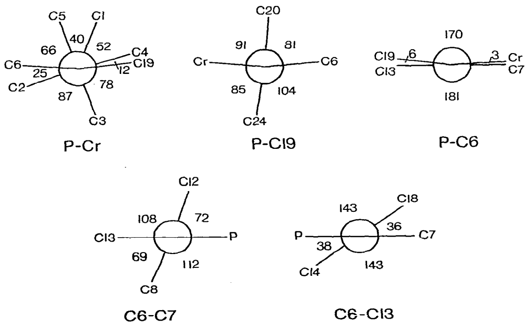
Fig. 2. Newman projections along the bonds of the phosphathene group.
