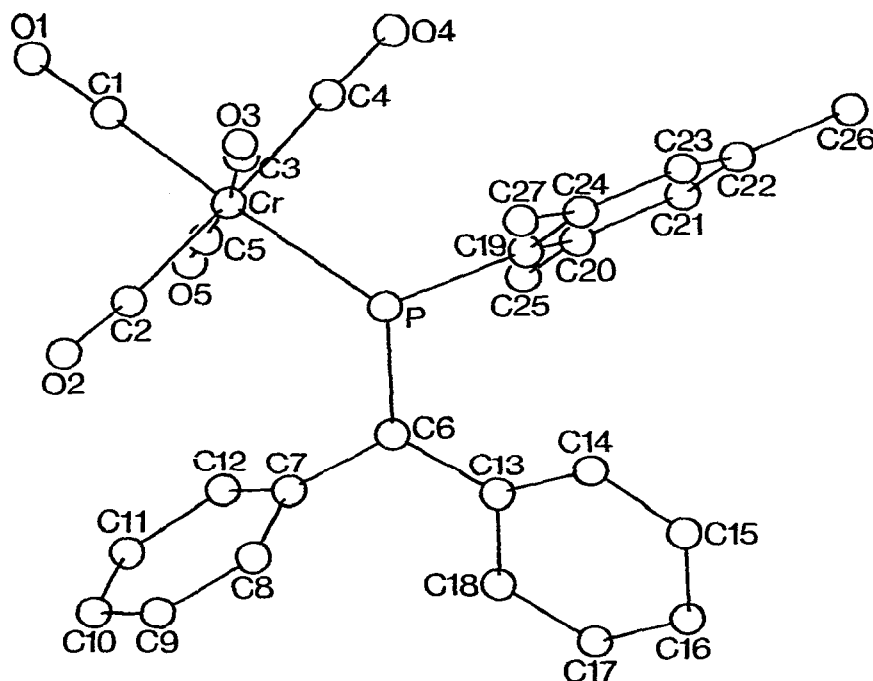
Fig. 1. Projection onto the plane of P, C(6), C(7), C(13), C(19) and Cr.
