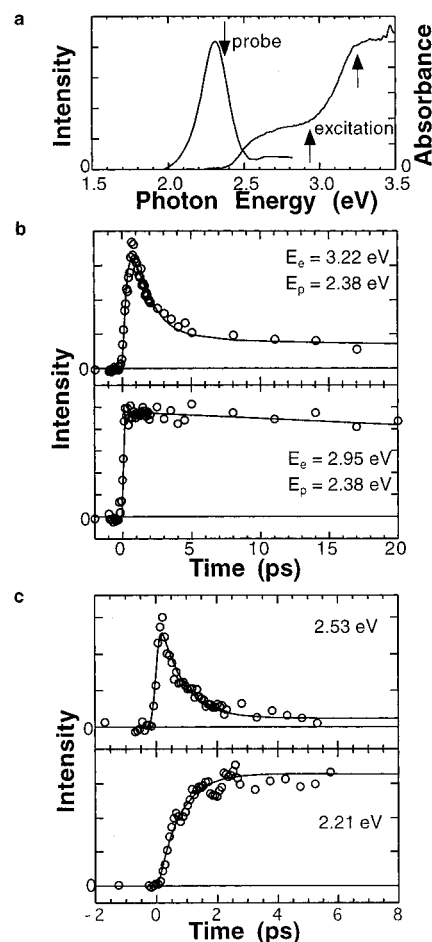
Figure 4. (a) Absorption and fluorescence spectra of MCISA 293 K. (b) Fluorescence decays of MCISA at 2.38 eV excited at 3.22 eV (upper) and 2.95 eV (lower) at 293 K. (c) Time dependence of the fluorescence of CISA at 77 K. The fluorescence energies are 2.53 (upper) and 2.21 eV (lower).
