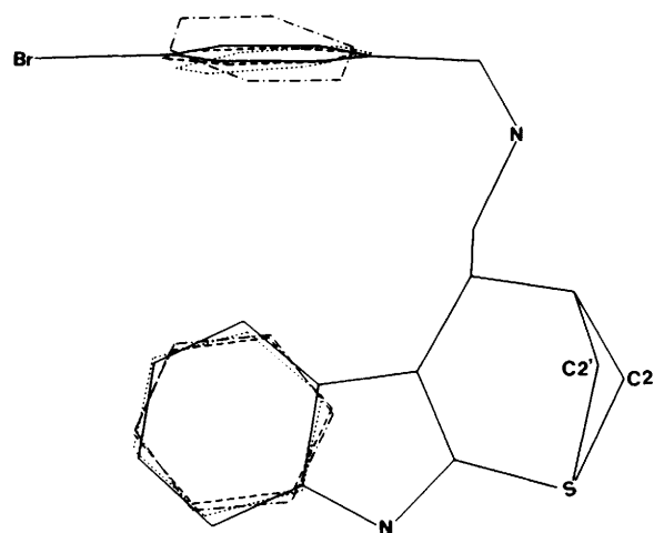
Figure 5. Comparison of (19) (bold line) and N -phenylacetyl-L-Phe (-----), L-Lys-L-Phe-L-Phe (.....), and benzoyl ester of L-Phe (.....). Each peptide molecule was superimposed to (19) by fitting at 12 points of two phenyl rings. Only phenyl rings are shown for clarity. The co-ordinates of these peptides were obtained from ref. 14a-c.
