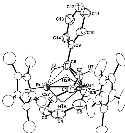
Figure 1. ORTEP drawing of 8' , with thermal ellipsoids at the 25% probability level. One disordered \text{C}_5\text{Me}_4\text{Et} ligand on Ru1 has been omitted for clarity. Selected bond lengths (Å), angles, and a torsion angle (deg): Ru1–Os1, 2.597(1); Os1–C7, 2.15(1); Os1–C8, 2.15(1); Ru1–C8, 2.56(1); C7–C8, 1.43(2); Ru1–H8, 2.2(1); C8–H8, 1.0 (1); C7–H7, 0.9 (1); Os1–C7–C8, 70.7(7); Os1–C8–C7, 70.4(7); Os1–C8–Ru1, 66.3(3); C1–C7–C8, 124(1); C7–C8–C9, 120(1); C1–C7–C8–C9, 134(1).
