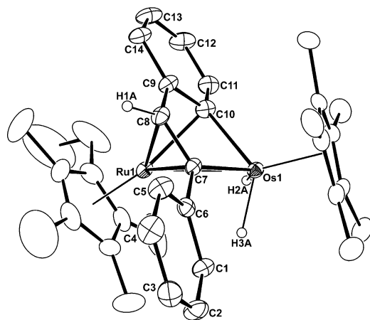
Figure 4. ORTEP drawing of 13' , with thermal ellipsoids at the 30% probability level. The second molecule in the unit cell has been omitted for clarity. Selected bond lengths ( \text{\AA} ) and angles ( ^\circ ): \text{Ru1-Os1} , 2.7564(5); \text{Os1-C7} , 2.107(5); \text{Os1-C10} , 2.085(6); \text{Ru1-C7} , 2.150(5); \text{Ru1-C8} , 2.185(5); \text{Ru1-C9} , 2.238(6); \text{Ru1-C10} , 2.183(6); \text{Os1-C7-Ru1} , 80.7(2); \text{Os1-C10-Ru1} , 80.4(2); \text{Os1-C7-C8} , 113.9(4); \text{C7-C8-C9} , 116.4(5); \text{C8-C9-C10} , 113.3(5); \text{Os1-C10-C9} , 114.6(4).
