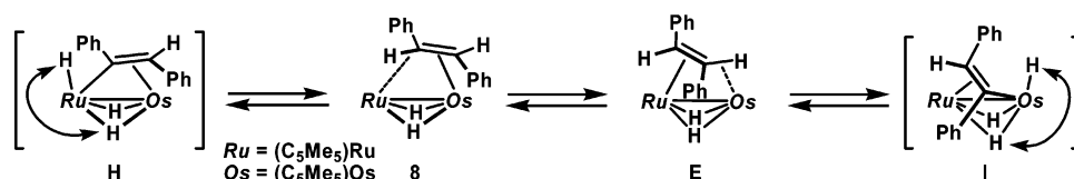
Scheme 3. Isomerization Reaction from Complex 10 to 8
