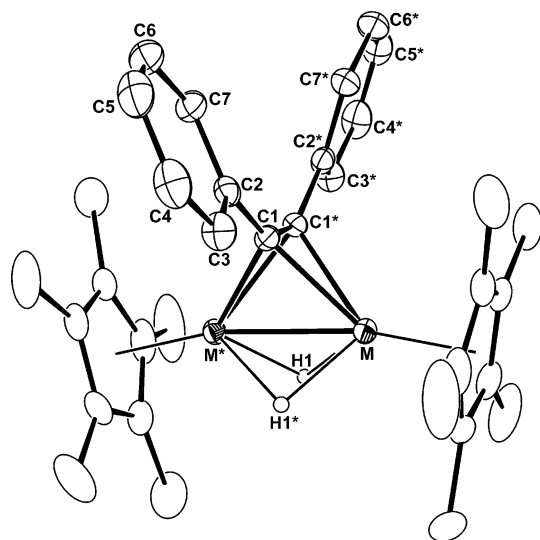
Figure 3. ORTEP drawing of 12 ( M = \text{Os} (50%) and \text{Ru} (50%)), with thermal ellipsoids at the 30% probability level. Selected bond lengths ( \text{\AA} ) and angles ( ^\circ ): M-M^* , 2.5433(7); M-C1 , 2.159(3); C1-C1^* , 1.323(6); M-C1-M^* , 72.20(9); C2-C1-C1^* , 141.6(2).
