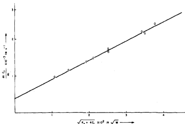
Figure 2. Dependence of the initial rate constant, dc/[(dt)c] , on [Br^-] [proportional to (K_s + 4c_1)^{1/2} ] for the isomerization of cis -PtBr(phenyl)(PEt 3 ) 2 in MeOH at 30 °C.
