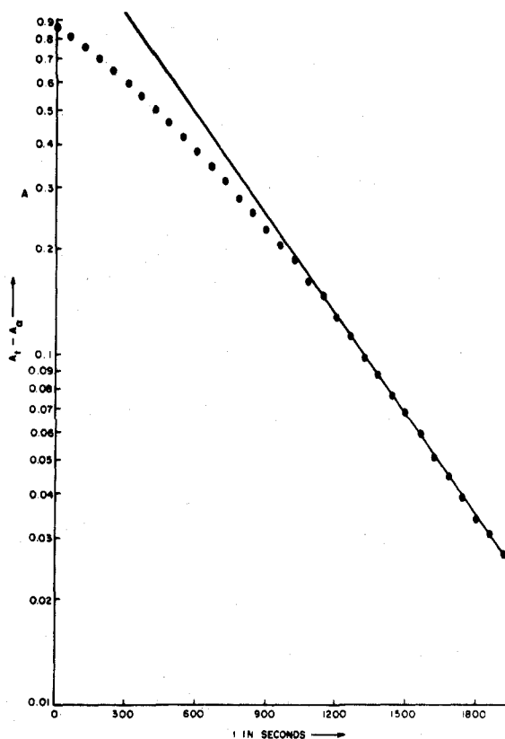
Figure 1. Graph of the logarithm of the absorbance change with time for the isomerization of cis - \text{PtBr}(\text{phenyl})(\text{PEt}_3)_2 in methanol at 30 °C. The initial complex concentration equals 3.08 \times 10^{-4} M.
