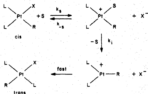
Scheme III
